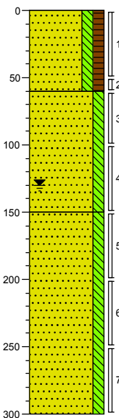
Boring: B02
