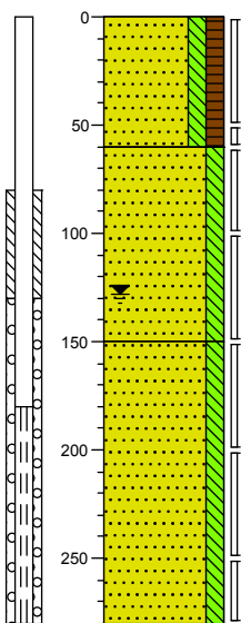
Boring: B01
